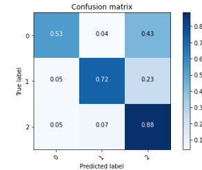
Figure 5: Confusion matrix of the results. 0 is Wake, 1 is REM, and 2 is NREM
