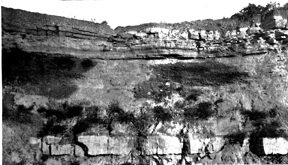
Fig. 1. Chanute shale, upper part.
