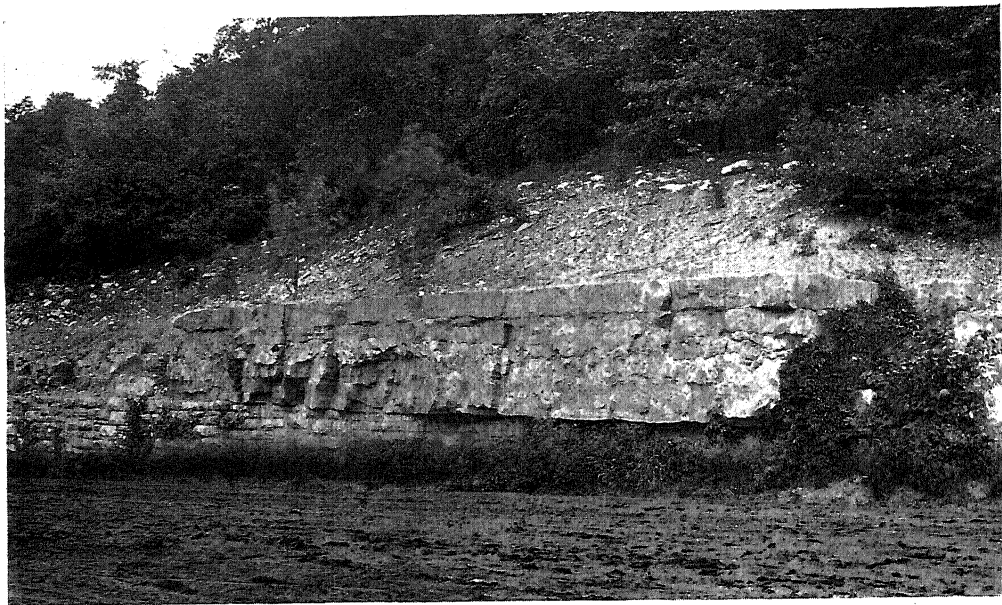
Fig. 1. Raytown limestone, Penn Valley Park.
