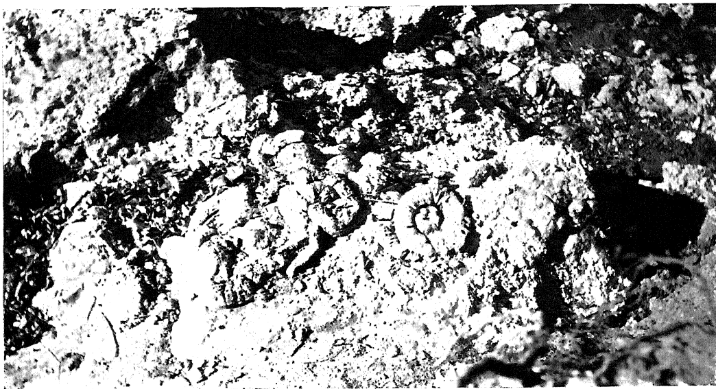
Fig. 1. Chaetetes in Pawnee limestone.
