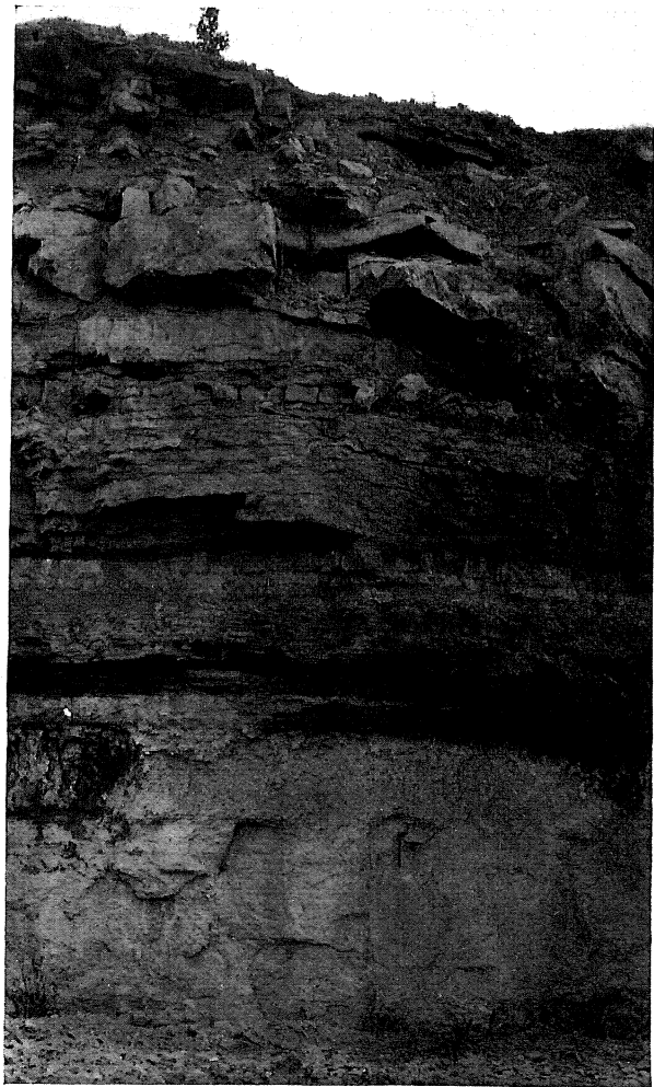
Fig. 1. Lower part of Winterset limestone, Galesburg shale
