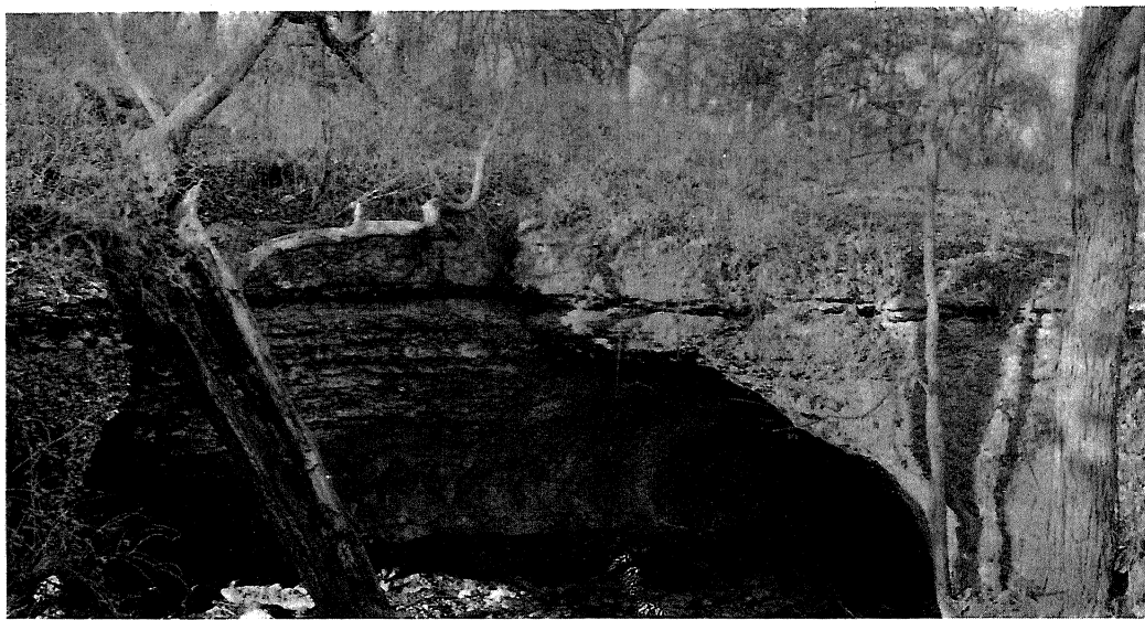
Fig. 2. Cave, Bethany Falls limestone, near Lees Summit.
